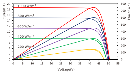
RSM132-8-750BHDG I-V characteristics at different irradiances
